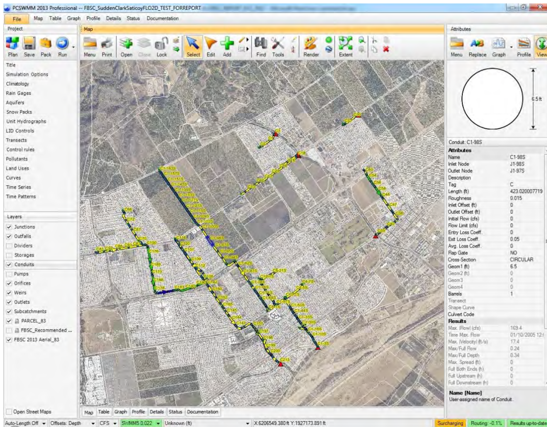
Figure 17 – EPA SWMM Model Schematic
